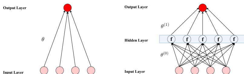
Figure 3.6: Neural Networks
