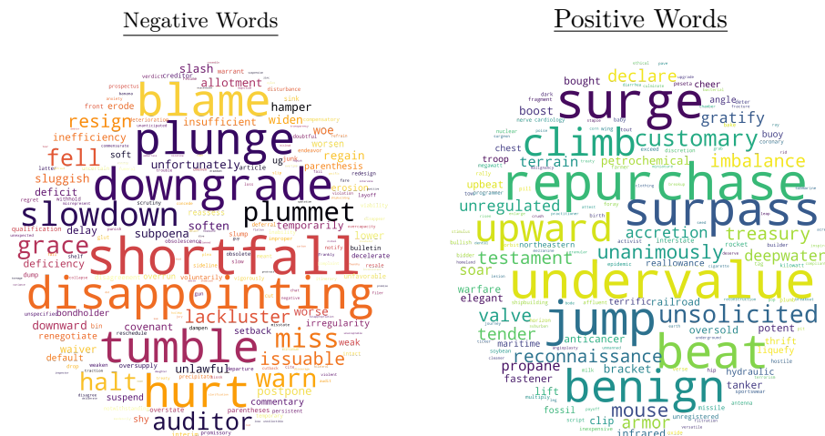
Figure 3.8: Sentiment-charged Words
